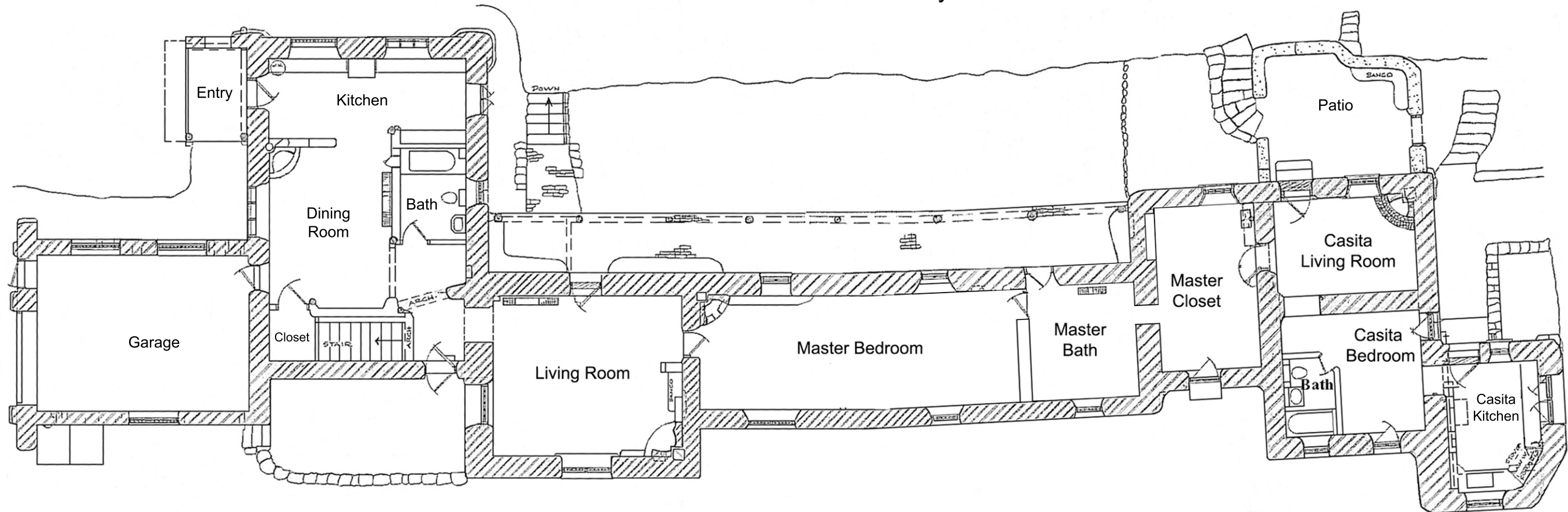
5 Cerro Gordo - Unit 5 & Unit 3 Floor Plan For Visual Aid Only
