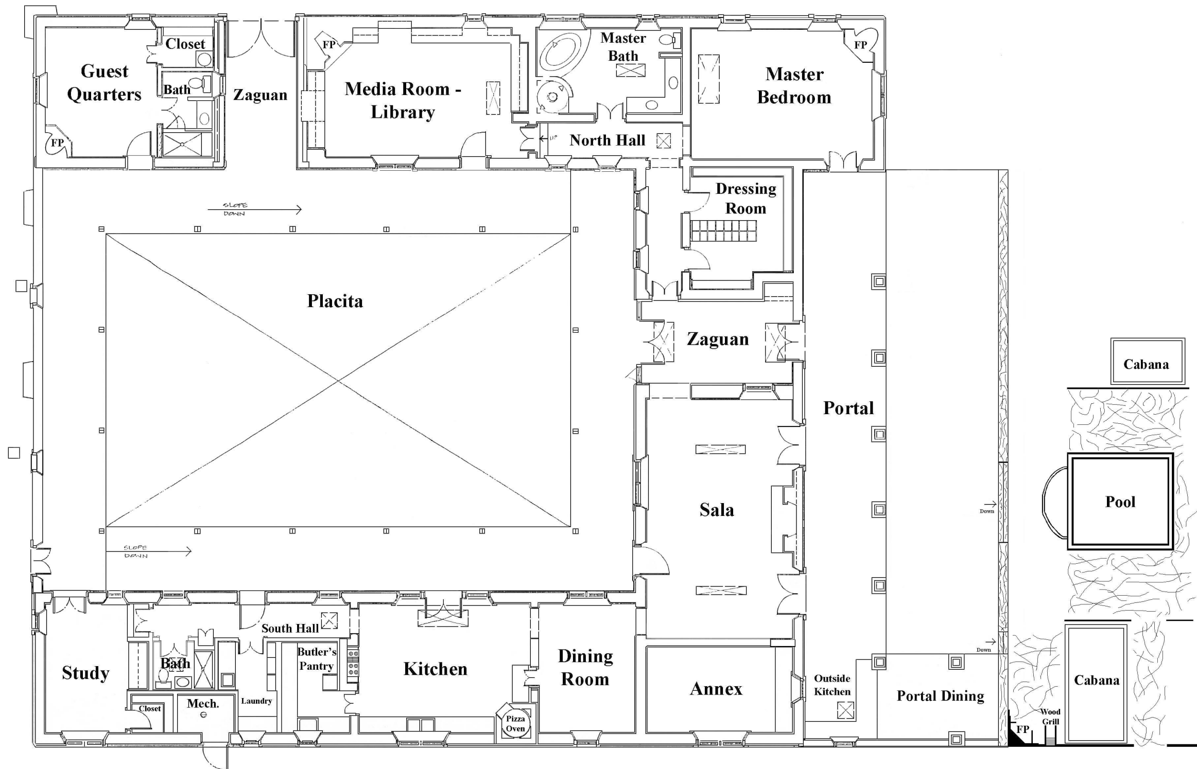
Apache Mesa Ranch 101 Mesa Prieta Rd. Main Residence - Floor Plan For Visual Aid Only
